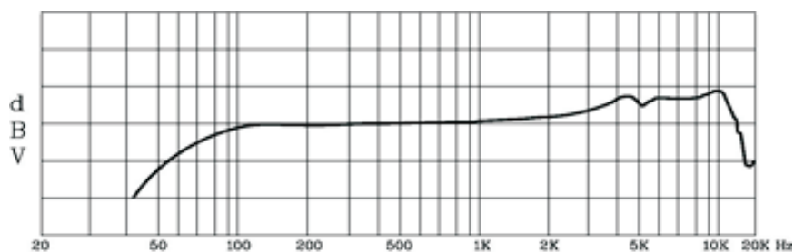
*Frequency Response
